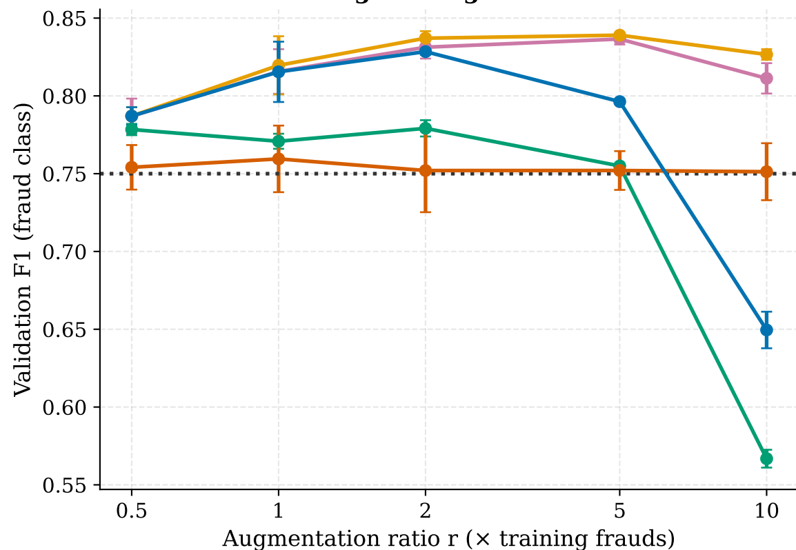
XGBoost (primary)
